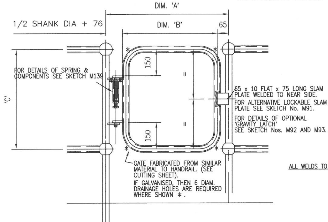
ELEVATION ON GATE (FROM PLATFORM SIDE).
