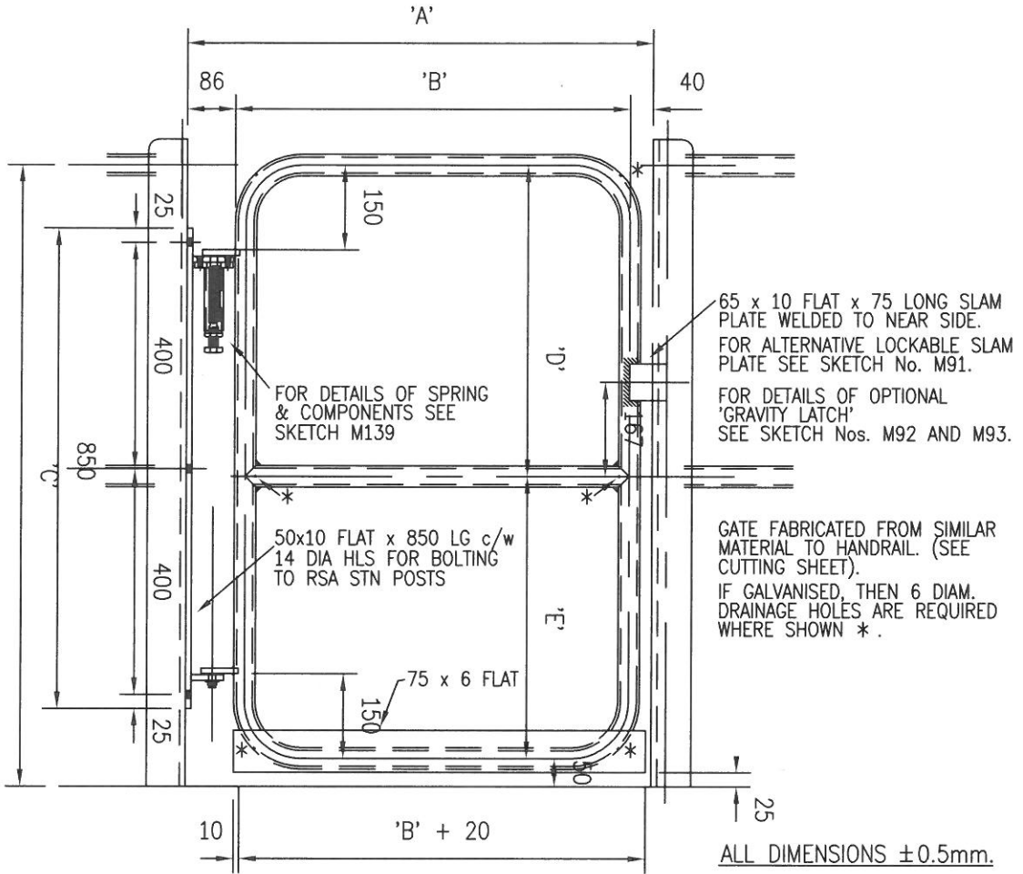
ELEVATION ON GATE (FROM PLATFORM SIDE).
